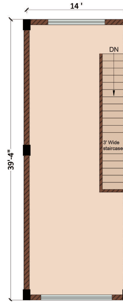
First Floor Plan Covered Area: 550 sq.ft. Floor to Floor Height: 15 ft.
