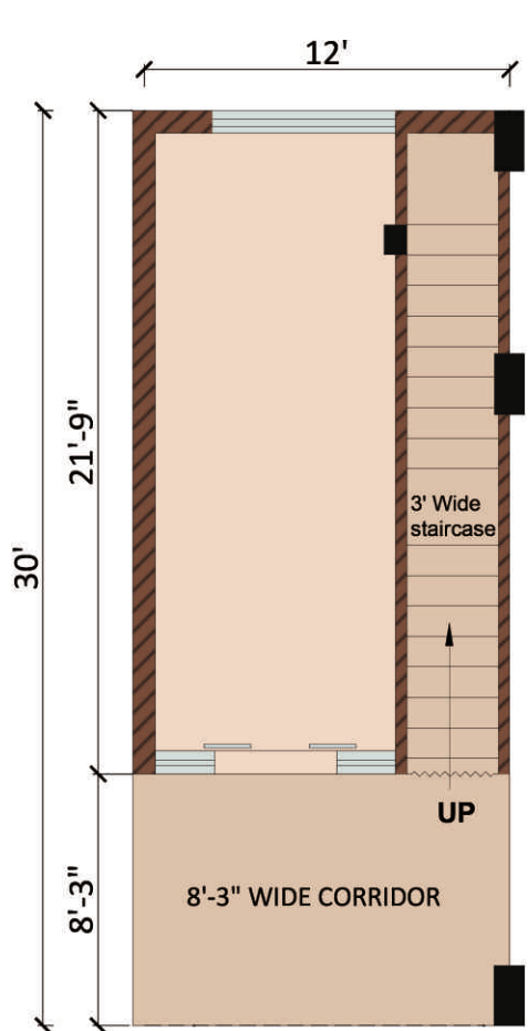
Ground Floor Plan Covered Area: 360 sq.ft. Floor to Floor Height: 11 ft.
