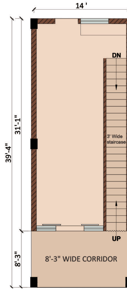
Ground Floor Plan Covered Area: 550 sq.ft. Floor to Floor Height: 11.25 ft.
