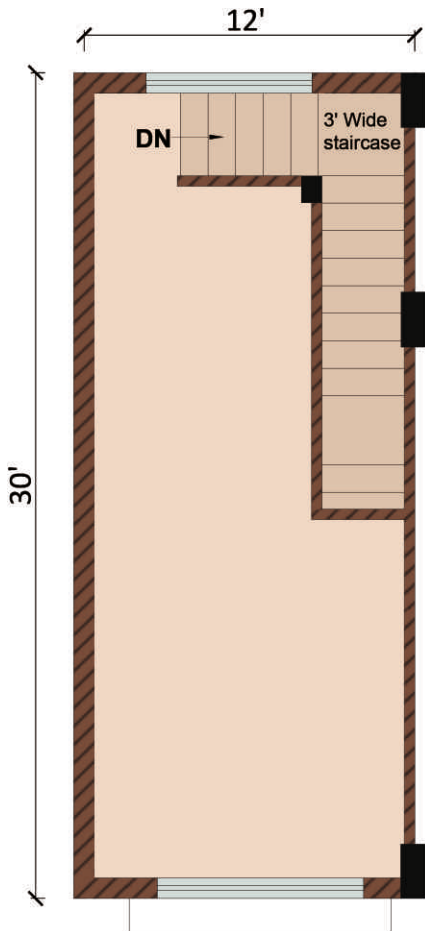
First Floor Plan Covered Area: 360 sq.ft. Floor to Floor Height: 14.25 ft.
